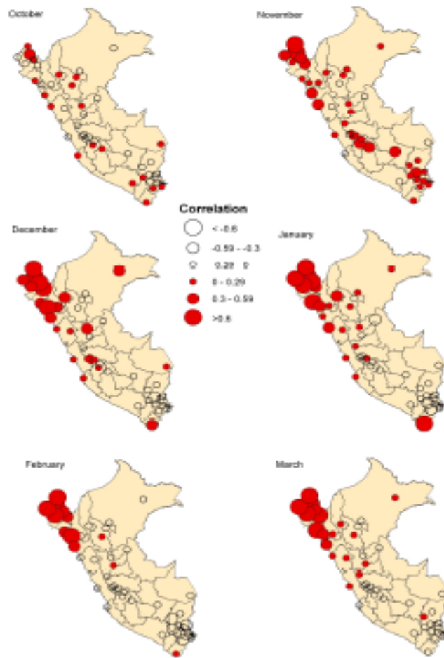
Fig. 3. Correlation between precipitation indices and SST anomaly indices in El Niño 1+2 region.
