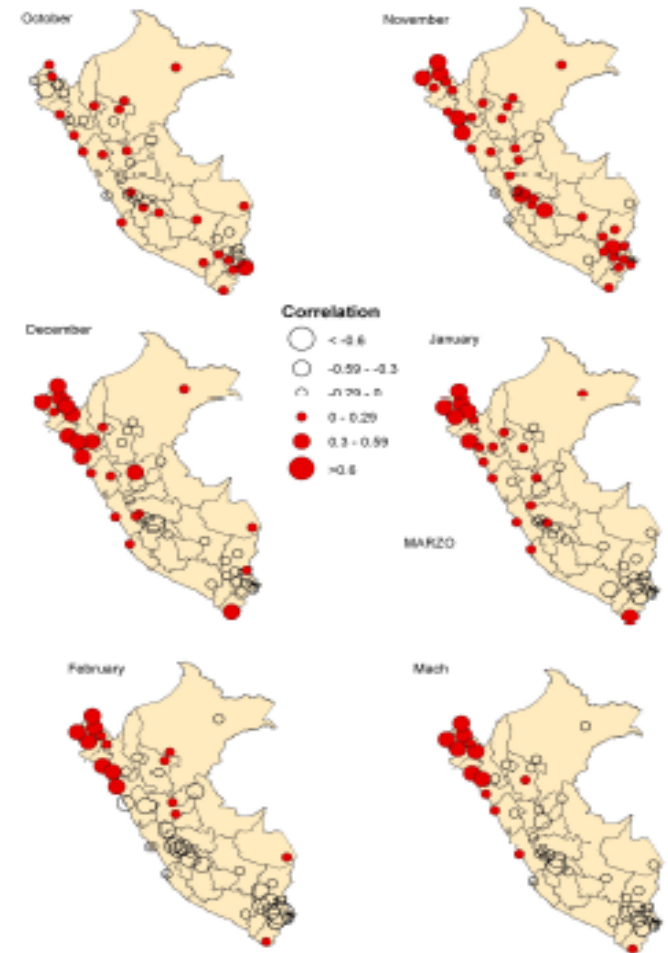
Fig. 4. Correlation between precipitation indices and SST anomaly indices in El Niño 3.4 region.
